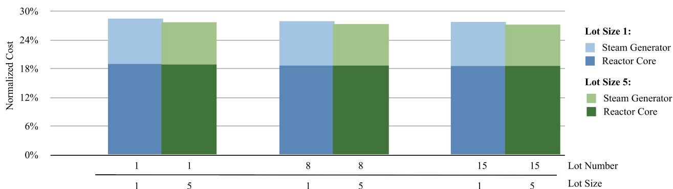
Figure 4: Normalized Cost Contributions – Reactor Core and Steam Generator Subcomponents.
