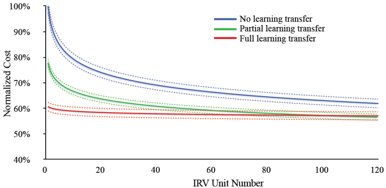
Figure 1: Normalized Cost as a Function of Credited Learning and IRV unit number.
